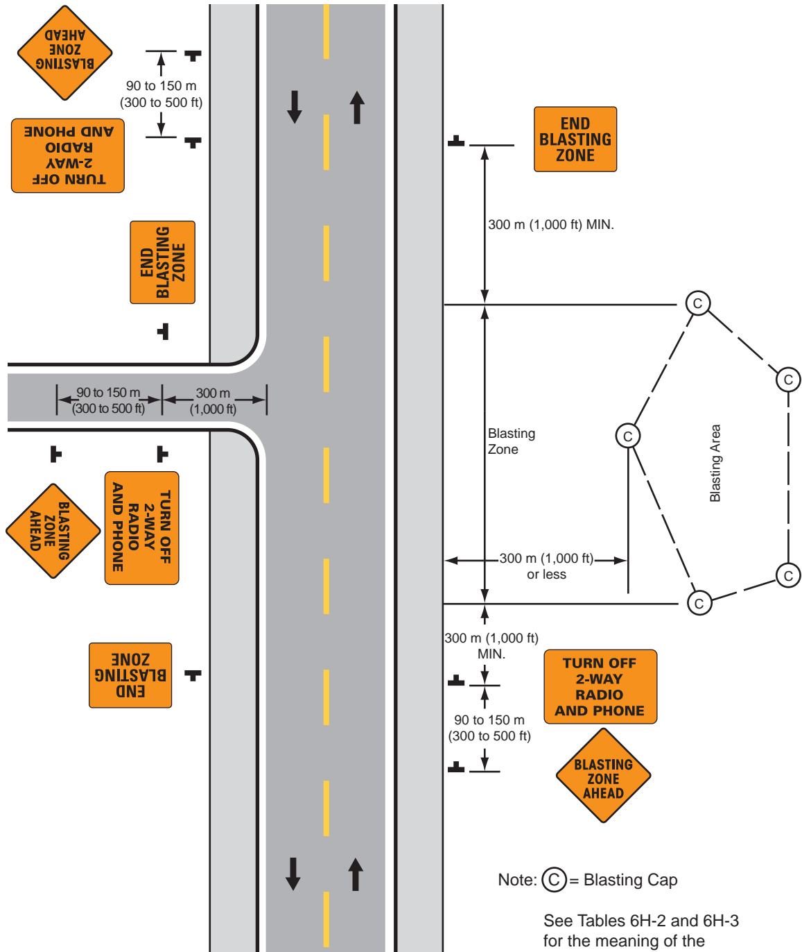
Figure 6H-2. Blasting Zone (TA-2)
